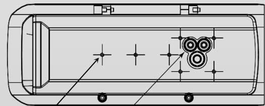
7 x 1/4-20 Threaded Mounting Holes 2 x 3/8" NPT 1 x 1/2" NPT Cordgrips
