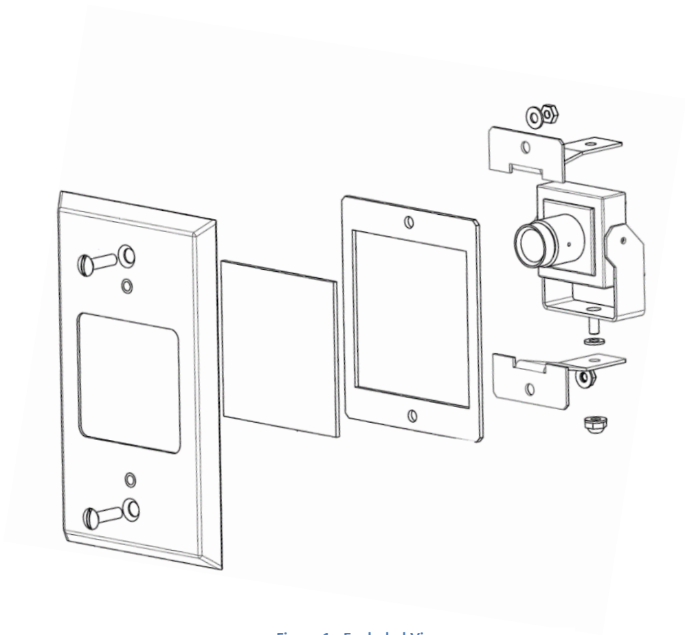
Figure 1 - Exploded View
